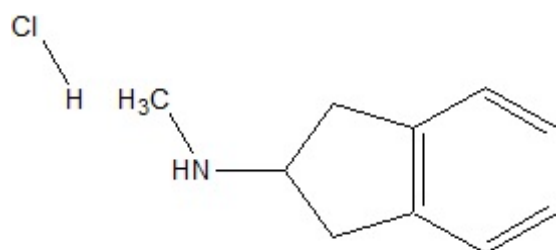
2-(methylamino)-indan hydrochloride
